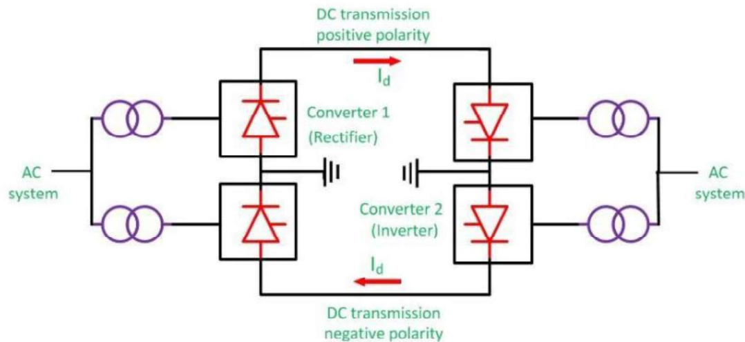
Fig.1. Schematic diagram of a bipolar system
