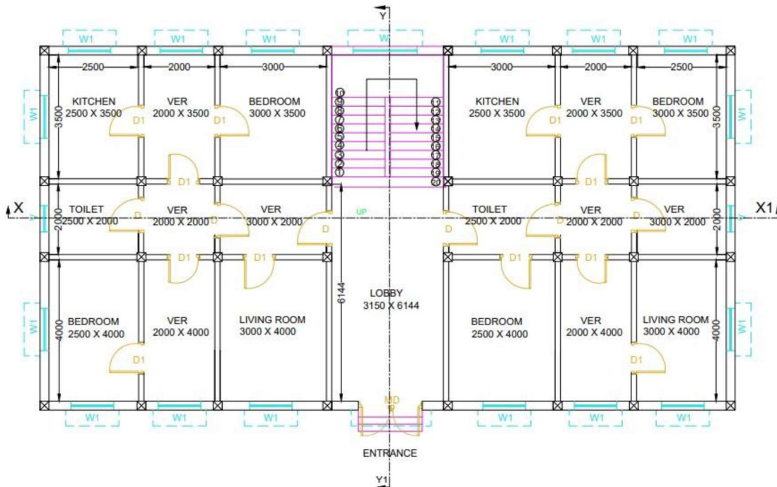
Fig. 3. Plan of Multi-storied building
