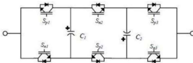
Fig.3 5 level X-SM structure
