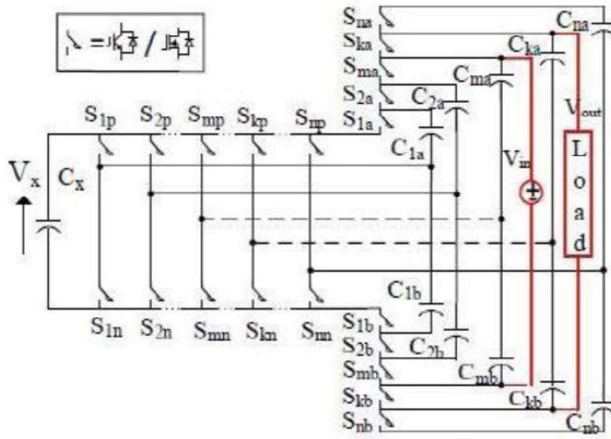
Fig.4 A generic (k/m) X Converter
