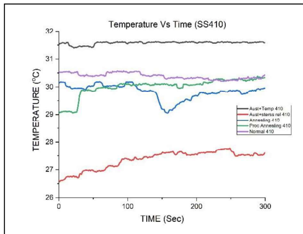
Fig 6: Temperature vs. time graph for SS410
