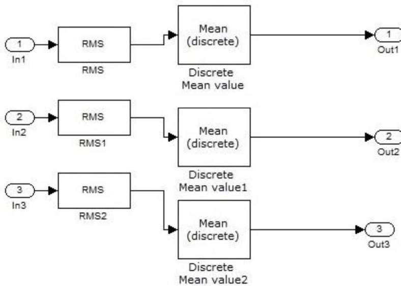
Fig 3.5: Subsystem of average voltage
