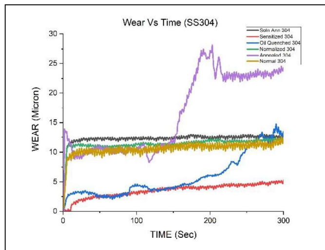
Fig 1: Wear vs. time graph for SS304
