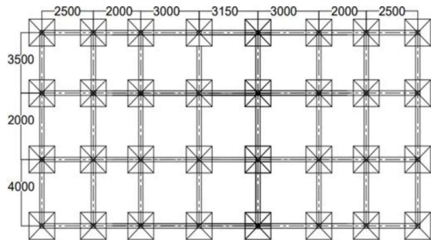
Fig. 2. Column & beam positions
