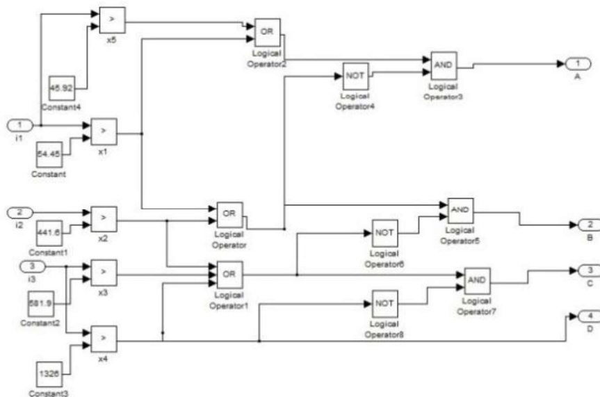
Fig 3.13: Subsystem of Instantaneous block
